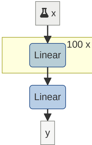
Vanishing Activations and Gradients
